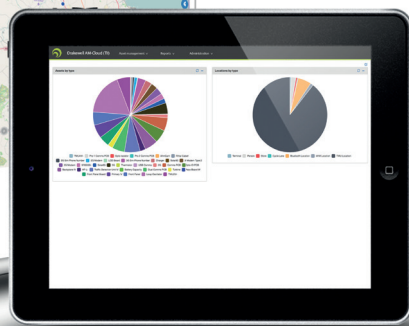
AM-Cloud dashboard
